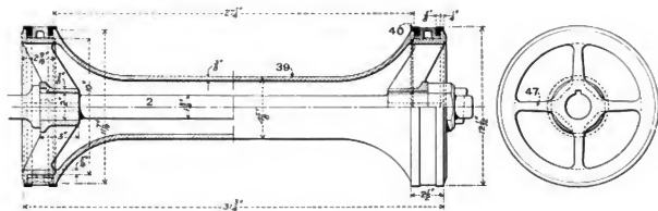
Figs. 2163-2164. Hollow Piston Valve. Northern Pacific.
